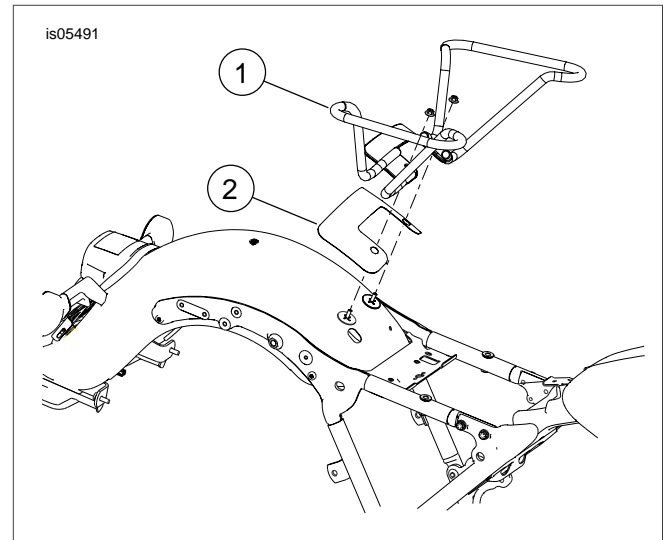
Figure 1. Service Parts: Passenger Grab Rail
