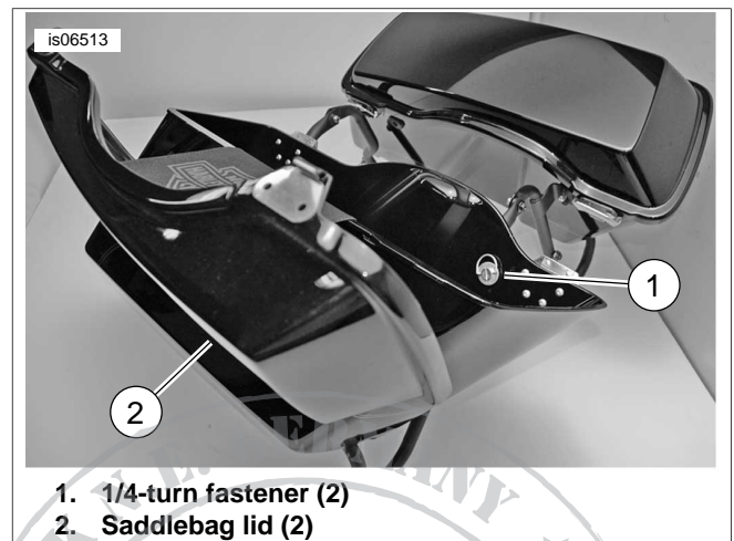
Figure 2. Install Saddlebags to Stand
