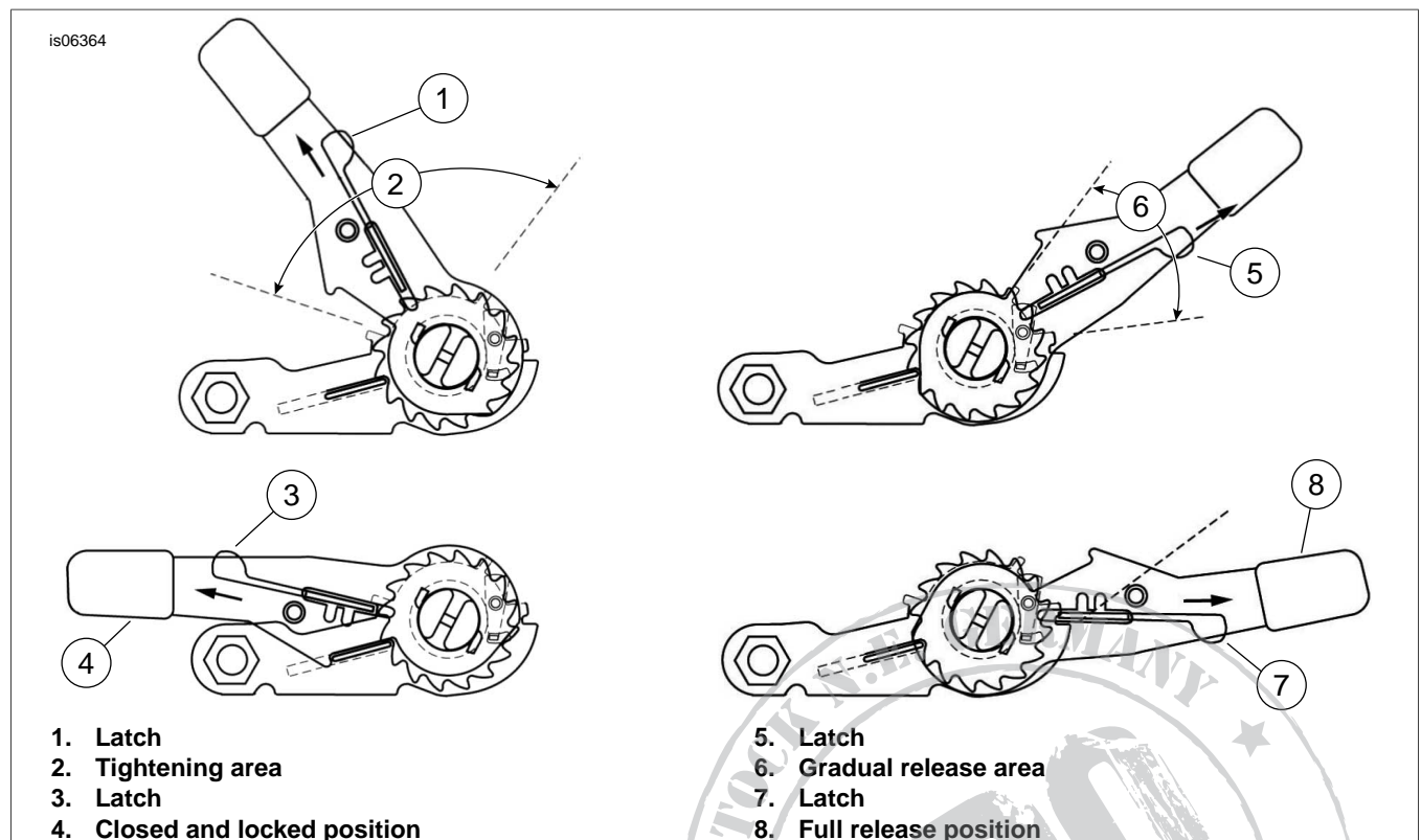
Figure 1. Slow Release Ratchet Strap
