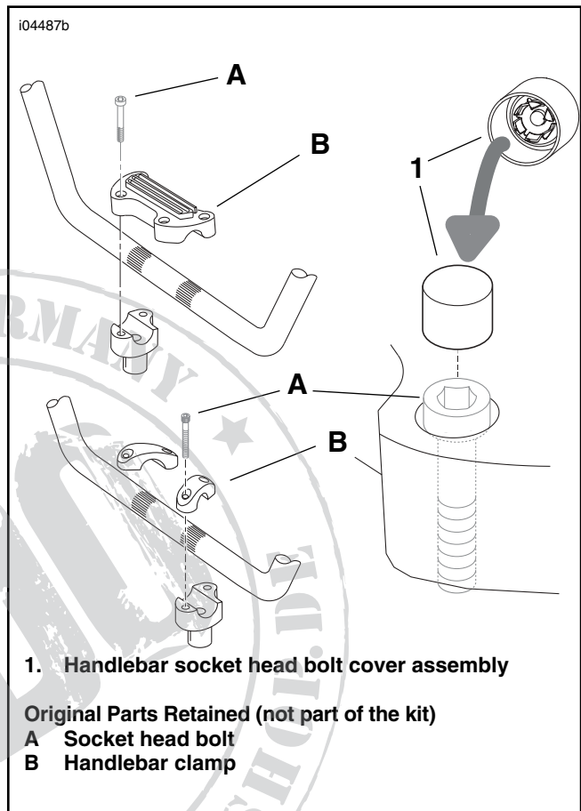
Figure 1. Handlebar clamp bolt cover
