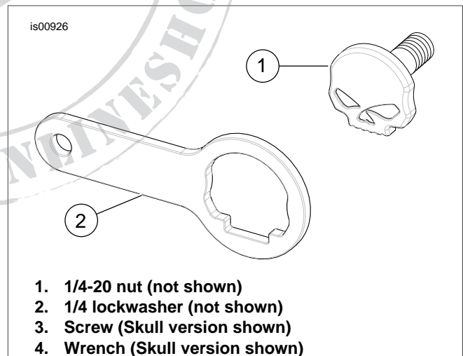
Figure 2. License Plate Hardware
