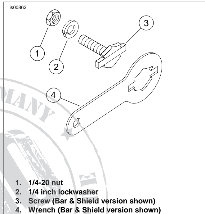
Figure 1. License Plate Hardware
