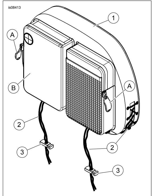
Figure 1. Service Parts: Rider Backrest Organizer Kit
