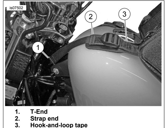
Figure 2. XL Tank Bag Front Straps
