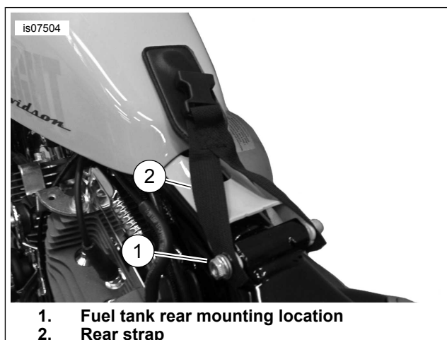
Figure 1. Rear Strap Installation
