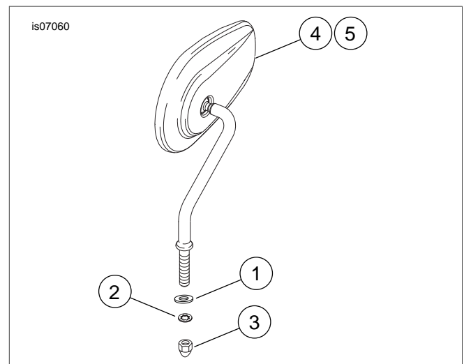
Figure 1. Service Parts: Mirror Hardware
