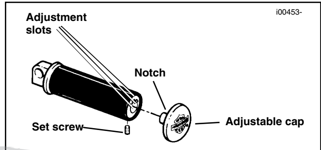
Figure 1. Exploded View - Small cushion footrest
