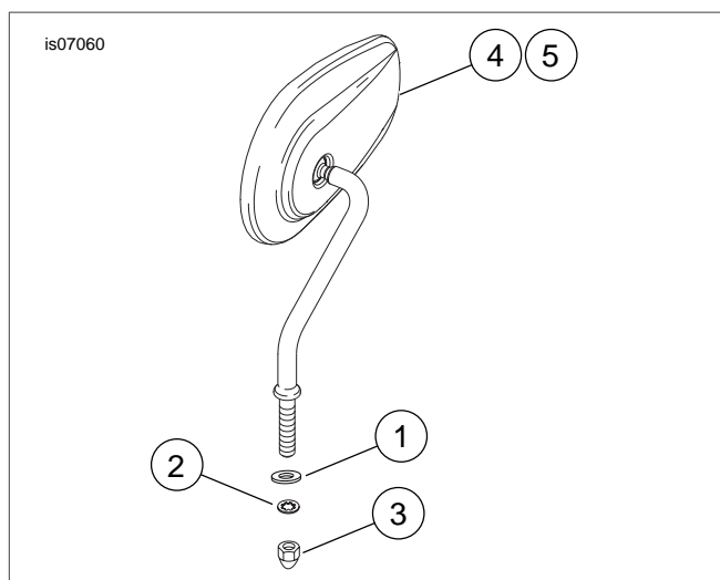
Figure 1. Service Parts: Mirror Hardware
