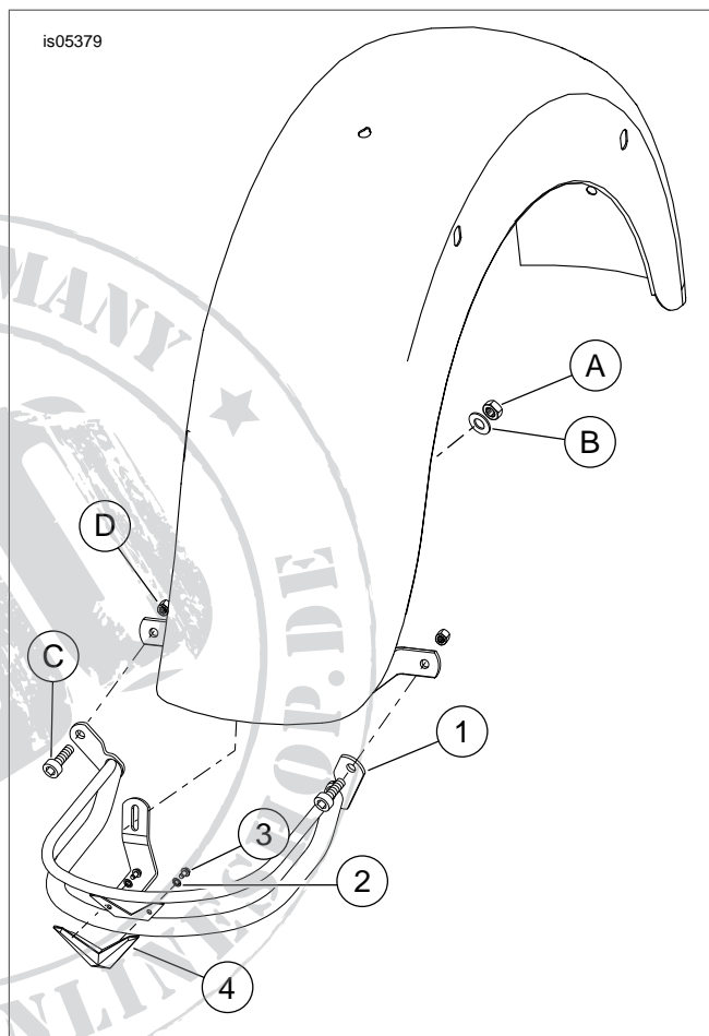
Figure 1. Service Parts: V-Logo Rear Fender Rail
