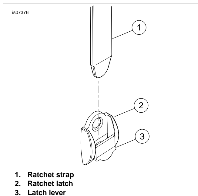
Figure 1. Ratchet Latch
