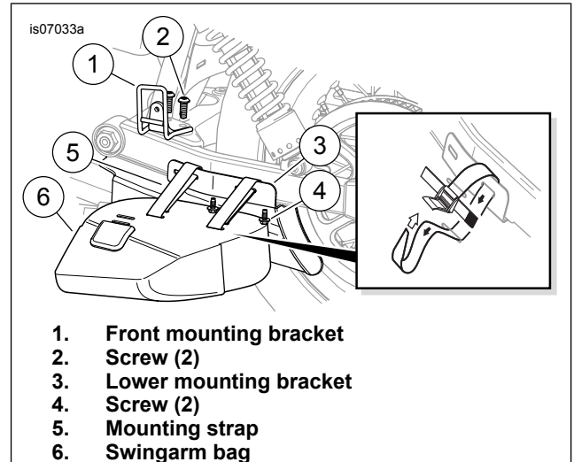
Figure 1. Install Saddlebag Brackets
