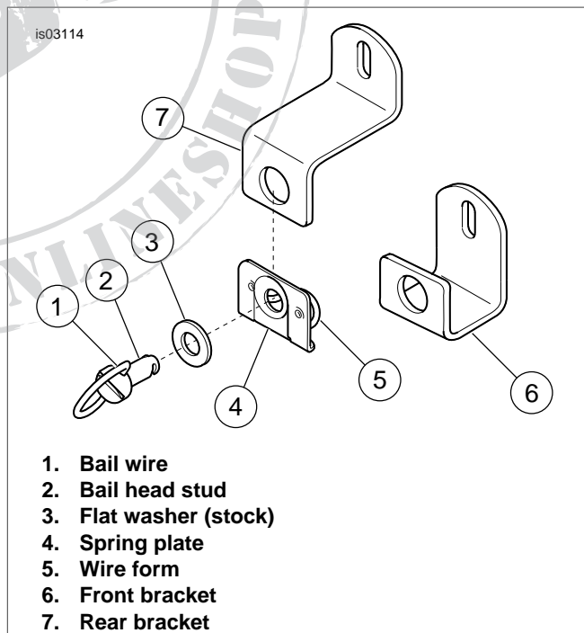
Figure 2. Saddlebag Quick-Release Fasteners
