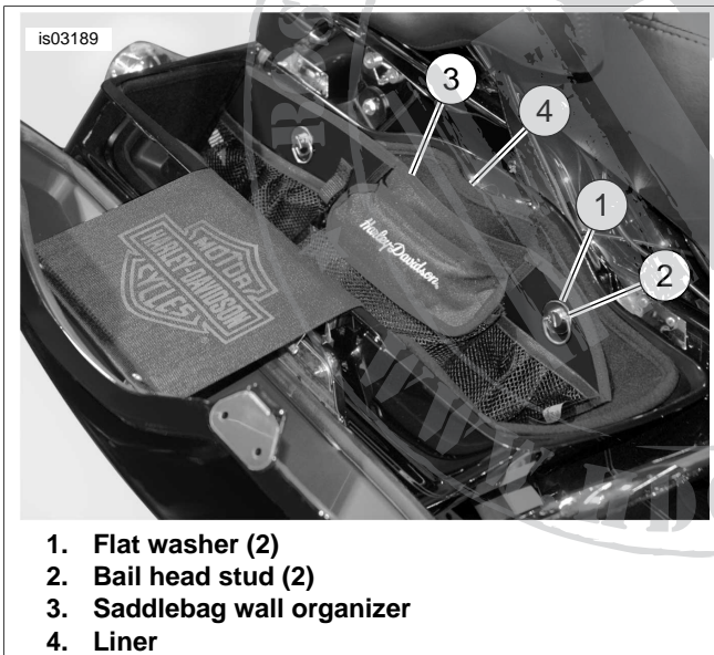
Figure 7. Install Saddlebag Wall Organizer (With Liner)
