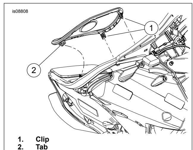
Figure 2. Install Speaker Grille
