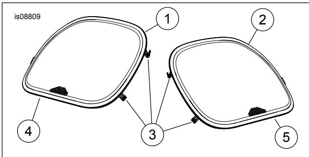
Figure 3. Service Parts, Boom! Audio 6.5 in Front Fairing Speaker Grille Kit
