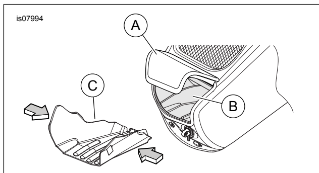
Figure 1. Media Storage Liner, Left Side
