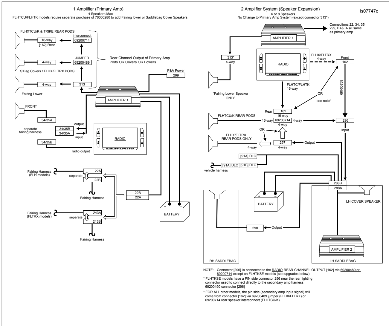
Figure 6. Amplifier Configuration
