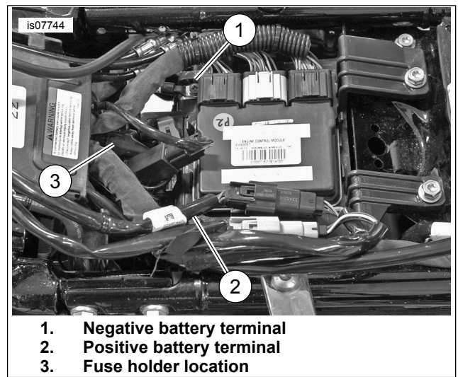
Figure 5. Battery Connection
