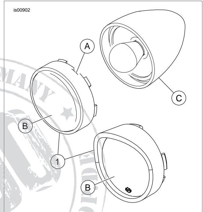
Figure 1. Bullet Turn Signal Trim Ring Kit
