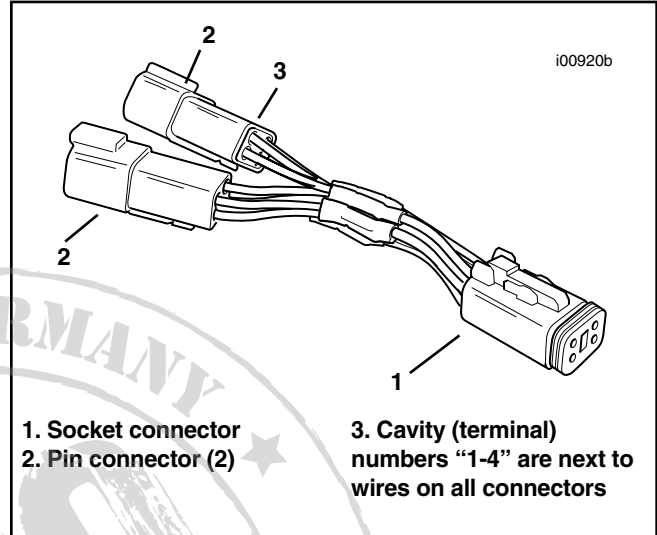
Illustration. Two-Into-One Harness Adapter
