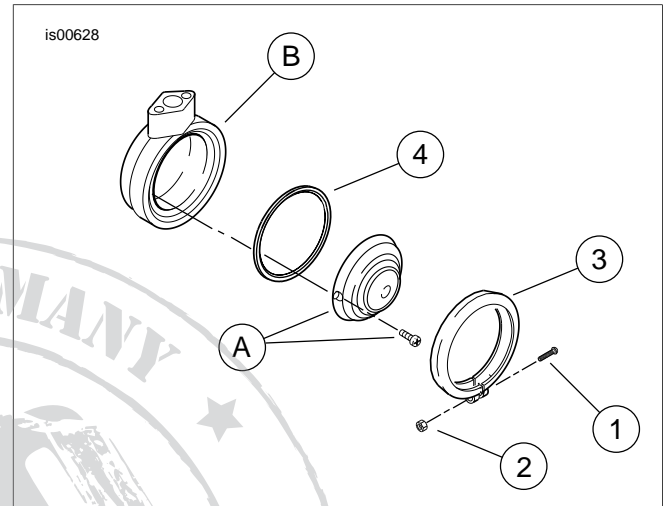
Figure 1. Service Parts: Turn Signal Trim Rings
