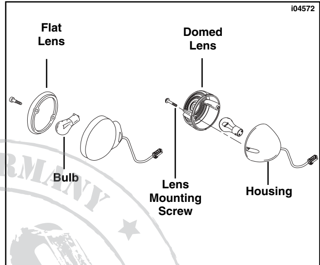
Figure 1. Flat and Domed Lens Turn Signals
