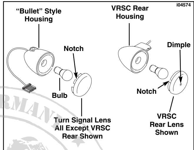
Figure 1. "Bullet" and VRSC Turn Signal Lenses
