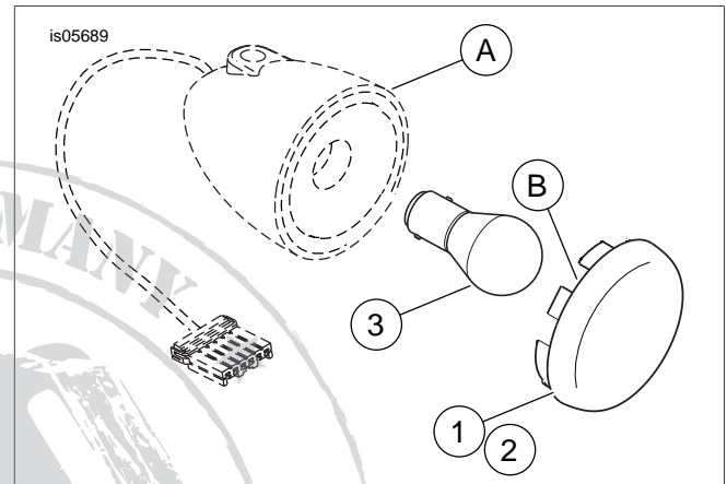
Figure 1. Service Parts: Bullet Front Turn Signal Lens
