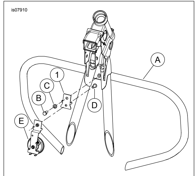
Figure 1. Service Parts: Horn Bracket Adapter Kit
