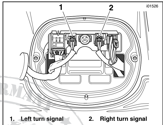
Figure 1. Turn Signal Connections
