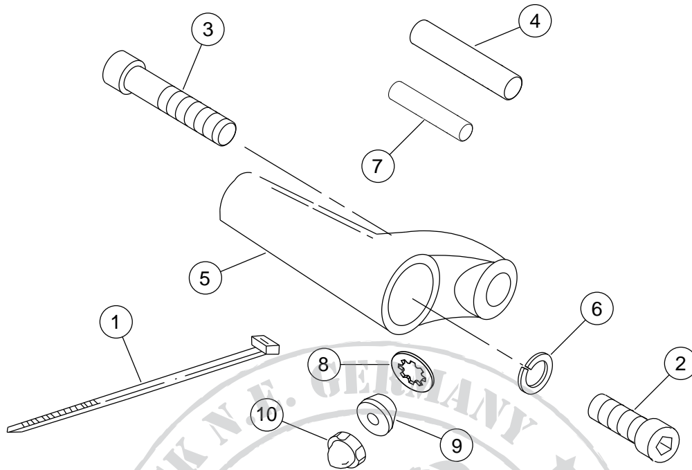
Figure 3. Service Parts: Front Directional Light Relocation Kit
