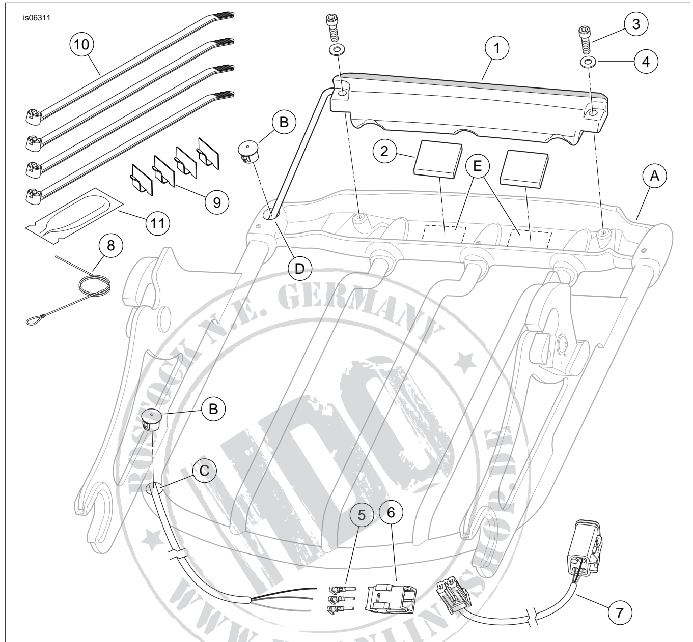
Figure 3. Service Parts, Air Wing Detachable Luggage Rack Light Kits
