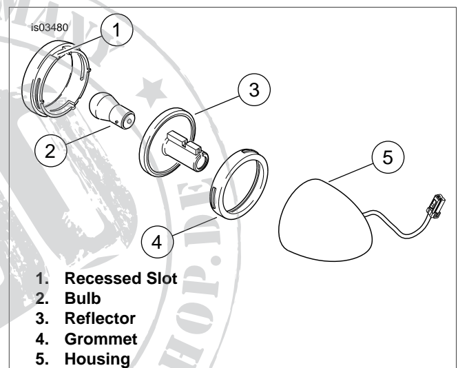
Figure 6. Lamp Assembly
