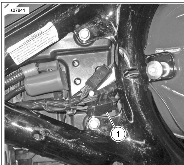
1. Rear Lighting Harness Connector [40A]
