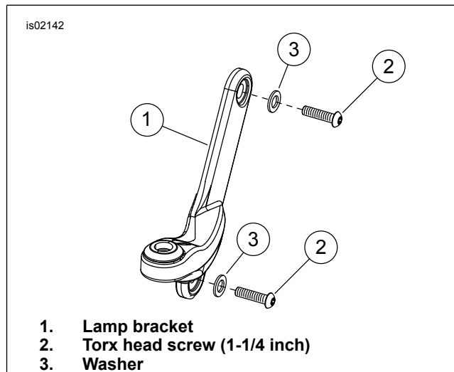
Figure 7. Lamp Bracket Assembly (left side shown bare)
