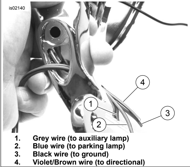
Figure 3. Directional Wiring Routing Shown
