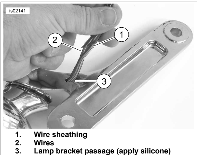
Figure 4. Installing Wire Sheathing
