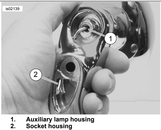
Figure 2. Lamp Wiring Routing Shown
