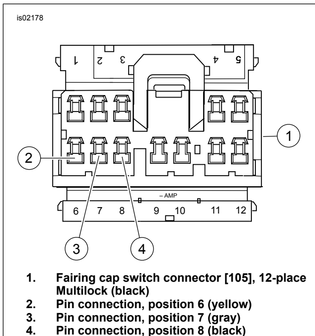
Figure 6. Fairing cap switch connections
