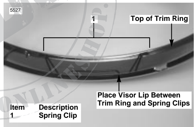
Figure 3. Spring Clip/Visor Placement
