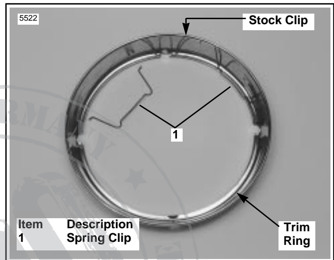
Figure 2. Spring Clips and Trim Ring
