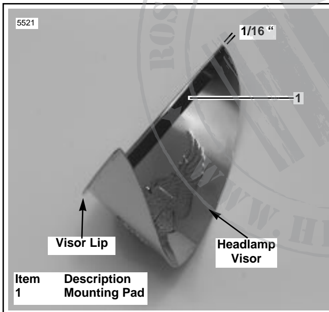
Figure 1. Visor Mounting Pad Attachment to Visor
