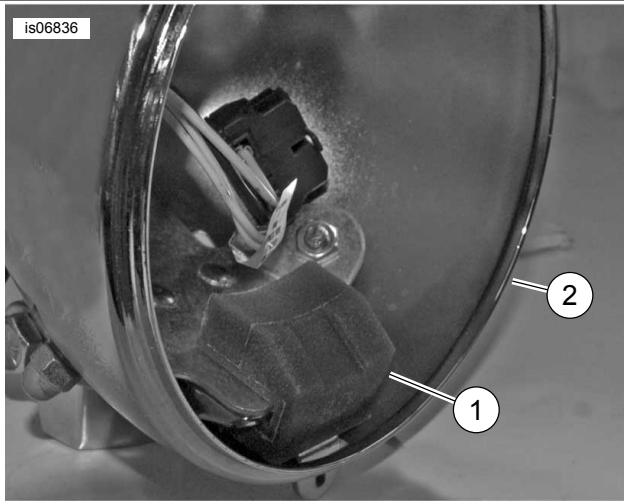
Figure 1. Install Headlamp Vibration Dampener
