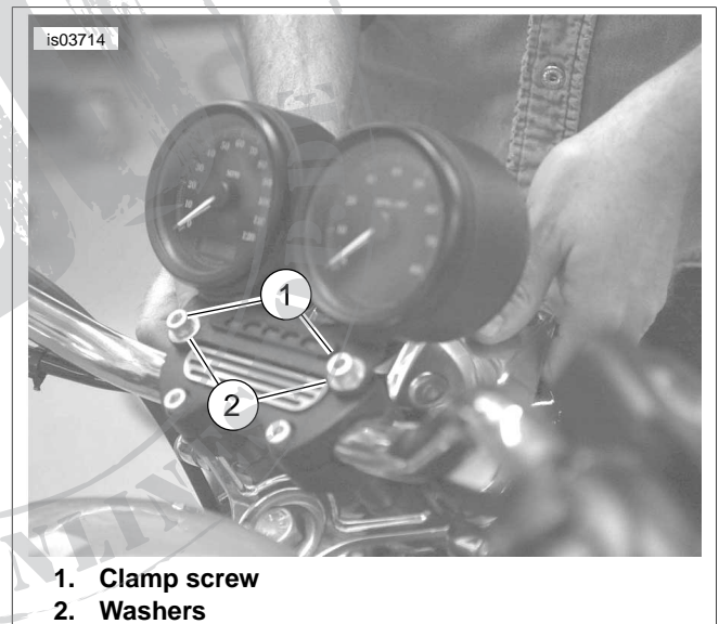
Figure 8. Install Speedometer/Tachometer Assembly
