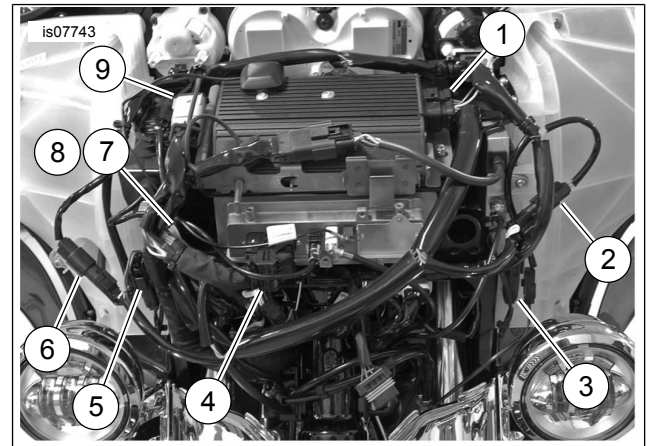
Figure 1. Service Parts: XL Black Header Pipes
