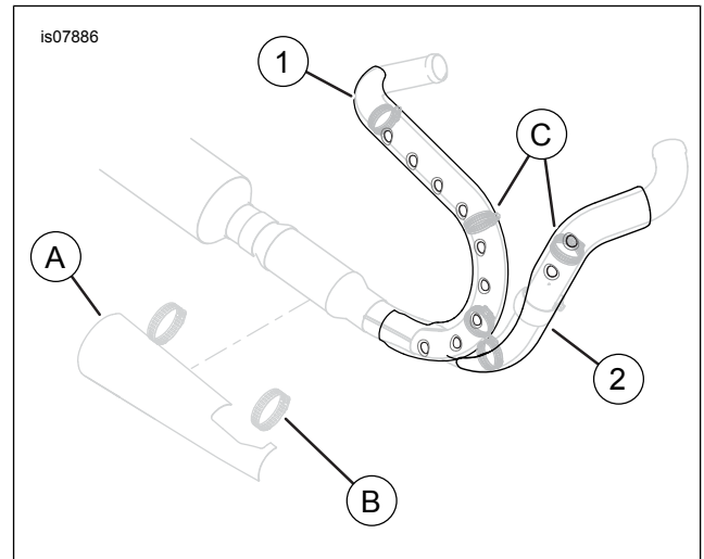
Figure 1. Service Parts: Exhaust Shield Kit
