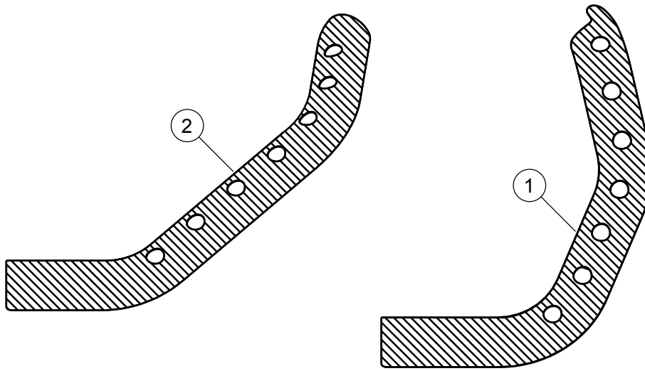
Figure 2. Service Parts: Sportster Exhaust Heat Shields
