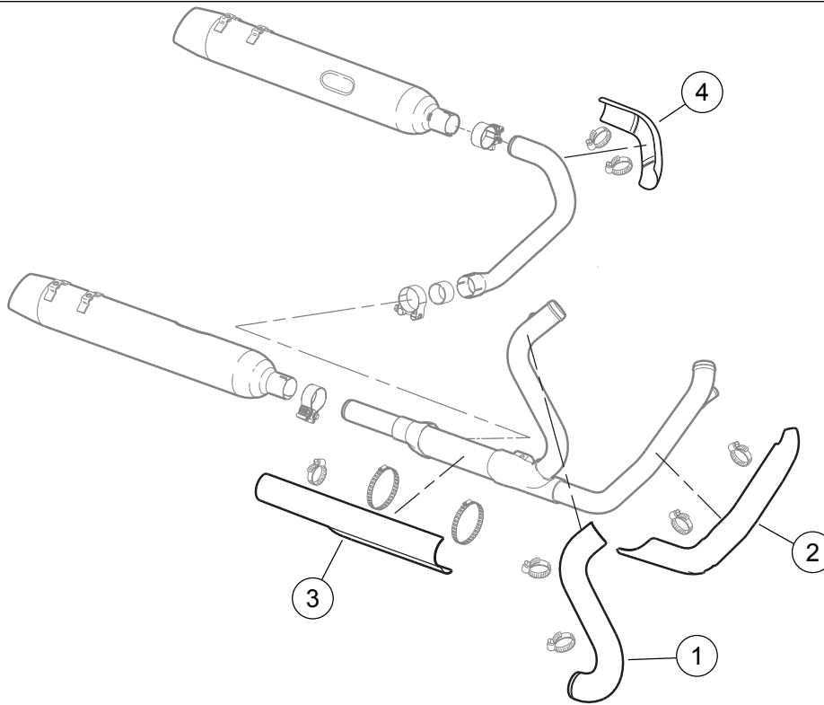
Figure 2. Service Parts: Touring Model P&A Exhaust Shields
