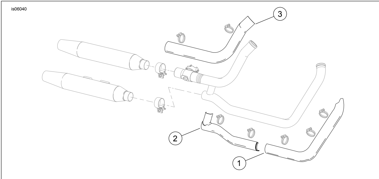
Figure 2. Service Parts: Softail Model Exhaust Shields
