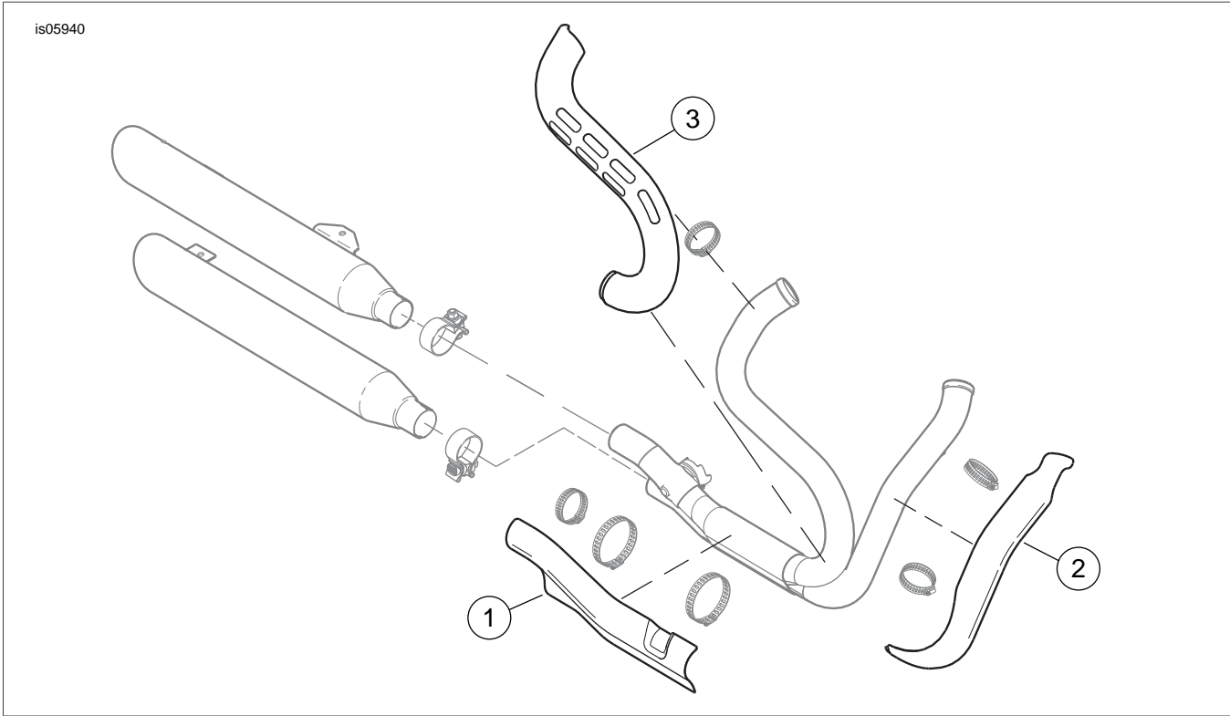
Figure 2. Service Parts: Dyna Model Exhaust Shields
