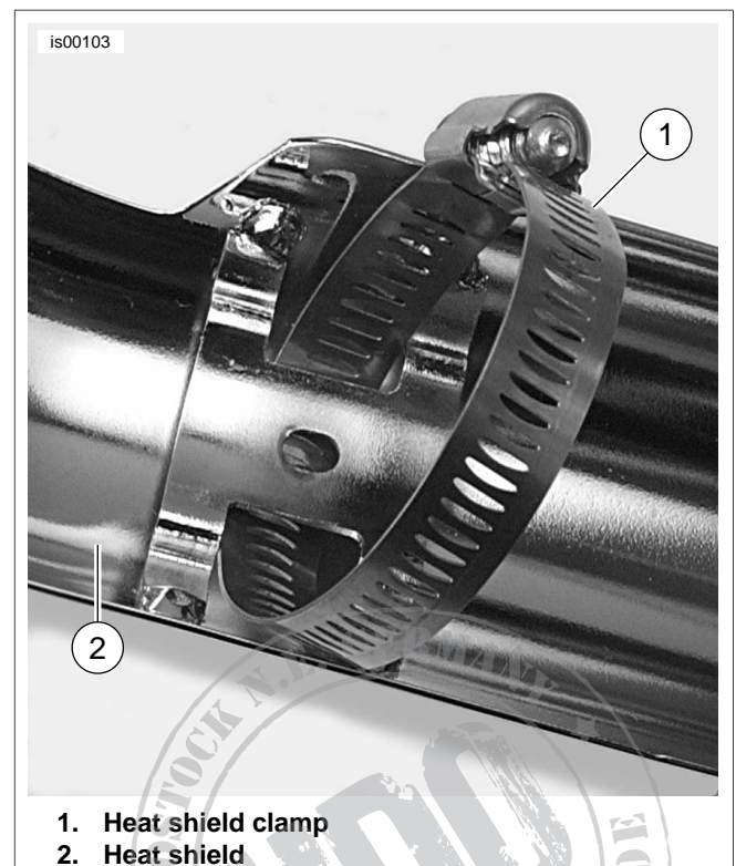
Figure 1. Heat Shield Clamp and Heat Shield
