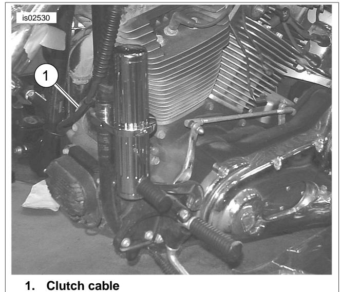
Figure 8. Mounting Location (Left Side of FXSTD Shown)
