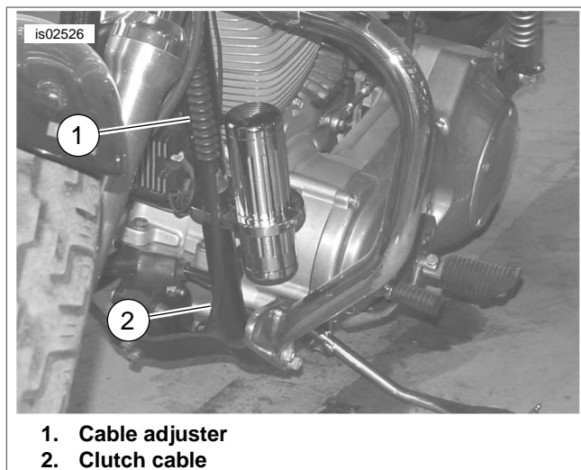
Figure 4. Mounting Location (Left Side of FXDX Shown)
