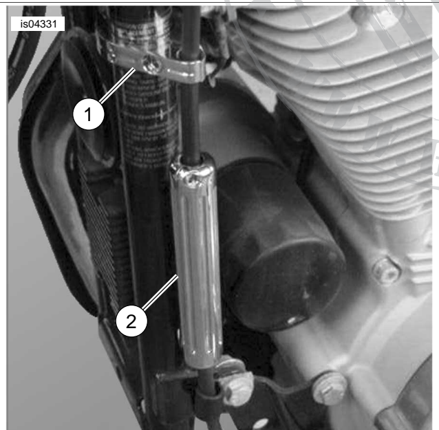
Figure 3. Install Clutch Cable Adjuster Cover, XL
