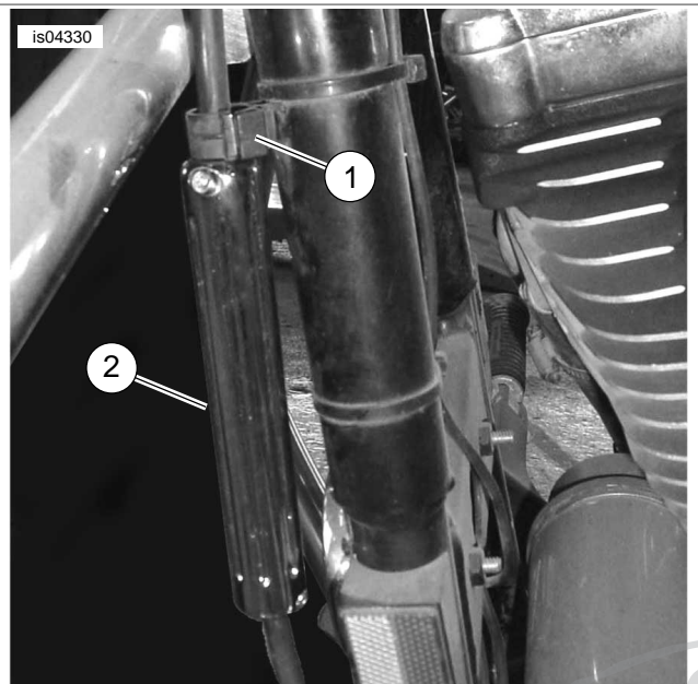
Figure 2. Install Clutch Cable Adjuster Cover, Dyna
