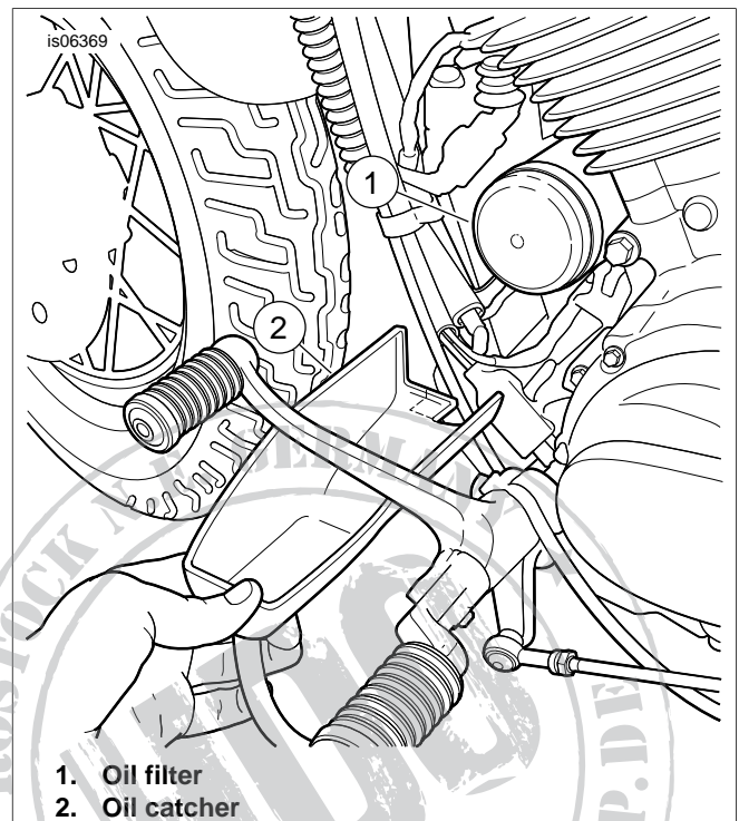
Figure 2. Oil Catcher
