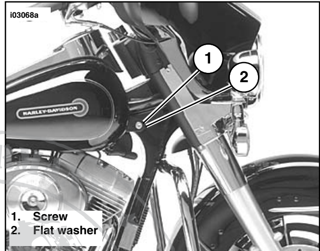
Figure 1. Fuel Tank Front Mount
