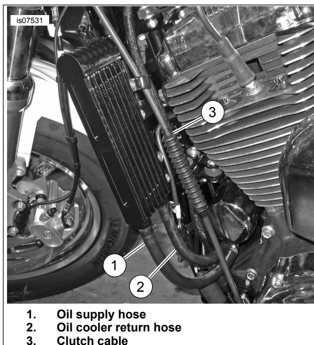
Figure 3. Oil Cooler Hose Routing
