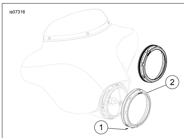
Figure 1. Burst Collection Trim Ring
