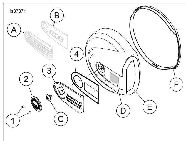
Figure 1. Service Parts: Air Cleaner Trim Kit
