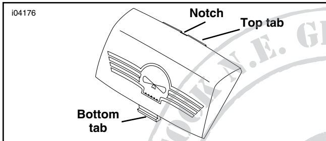
Figure 1. Fender-Tip Lens
