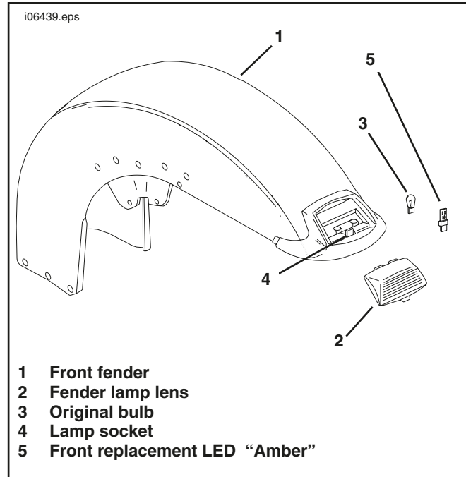
Figure 1. Front Fender Assembly Shown
