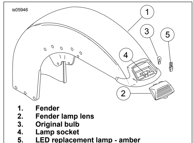
Figure 1. Front Fender Assembly
